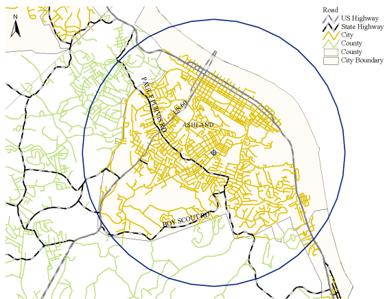
Neighborhood Scale: Air Toxics, Ozone, Sulfur Dioxide
