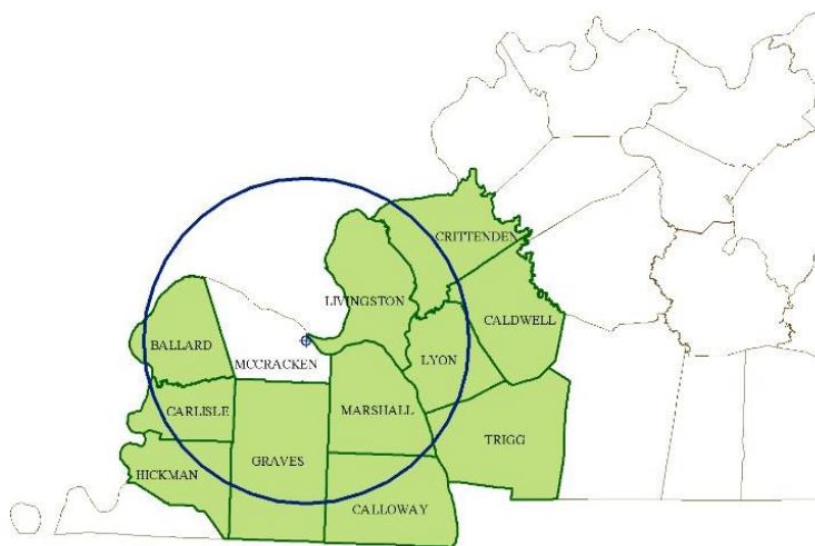
Urban Scale: Nitrogen Dioxide
