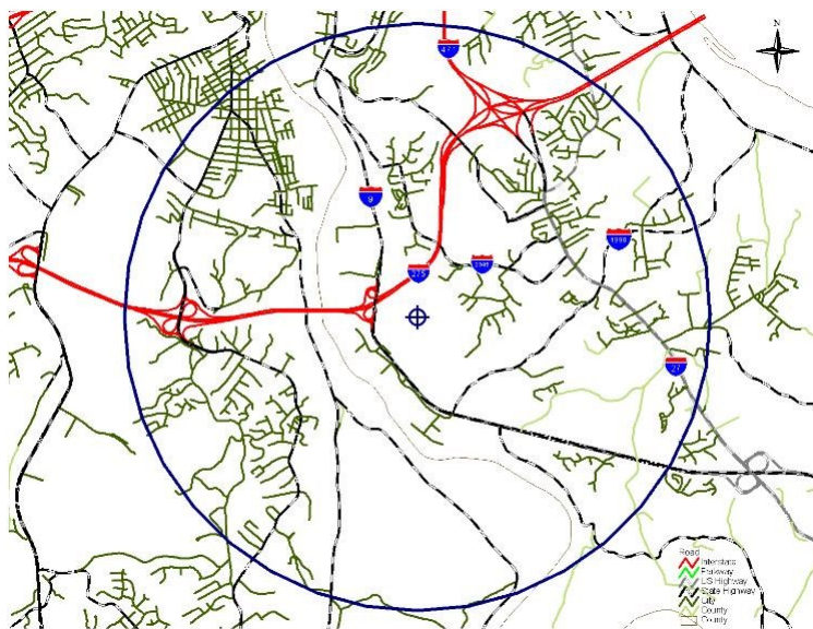
Neighborhood Scale: Particulates
